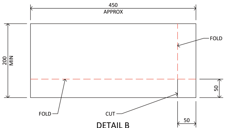
DETAIL B STRIP SCRIM REINFORCEMENT
