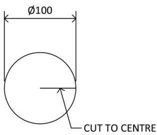
DETAIL A CIRCULAR CORNER SCRIM REINFORCEMENT
